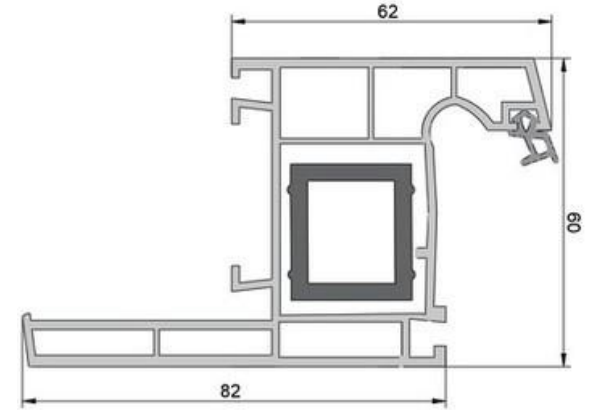
ES 060 Pervazlı Kasa Profili Super Renovation Frame Profile
