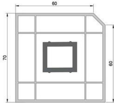
OP 09 Kutu Profili Box Profile (60x70mm)
