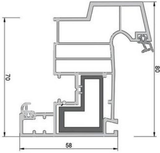
OKS 070 Damlalıklı Kanat Profili Window Drop Sash Profile
