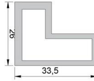
OP 13 Destek Profili Support Profile (33,5x26mm)
