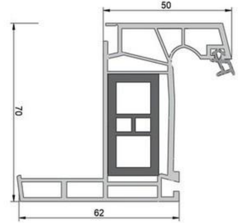
OKS 060 Pervazlı Kasa Profili Renovation Frame Profile
