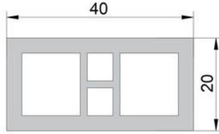
OP 12 Destek Profili Support Profile (40x20mm)
