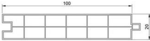
OP 04 Kapı Lambri Prof. Door Panel Profile ( lambri) (100x200mm)
